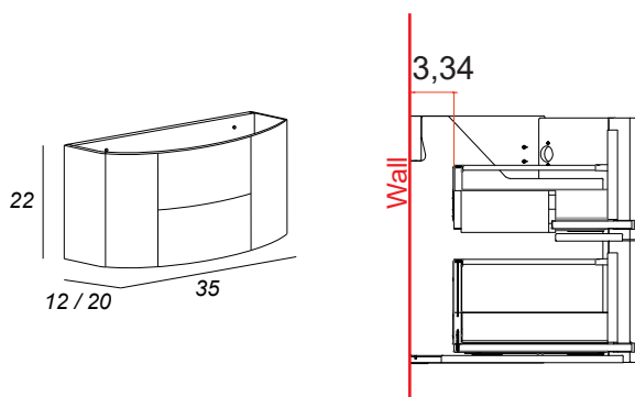
Side view for plumbing
