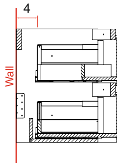
Side view for plumbing
